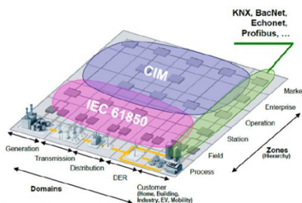
Fig. 2: SGAM standards mapping
