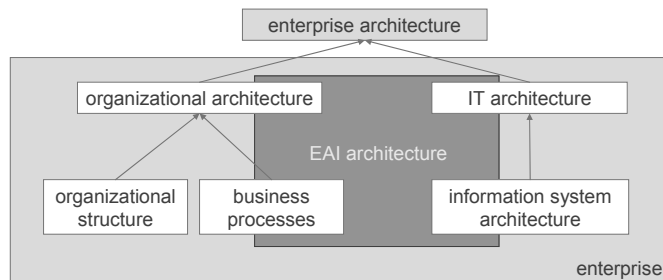
Fig. 2: Enterprise Architecture [14]
