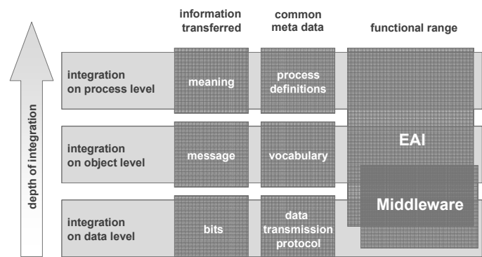
Fig. 1: Integration level [6]
